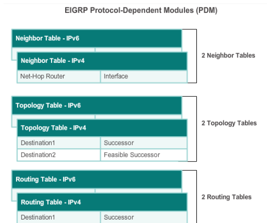
Figur: Protocol Dependent Modules[2014snc]
