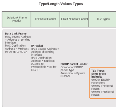
Figur: EIGRP inkapsling [2014snc]
