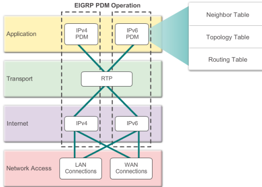
Figur: Reliable Transport Protocol[2014snc]
