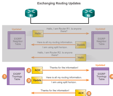
Figur: Informationsutbyte[2014snc]
