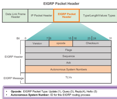
Figur: EIGRP Header [2014snc]
