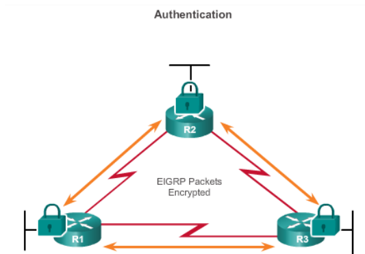
Figur: Authentisering[2014snc]
